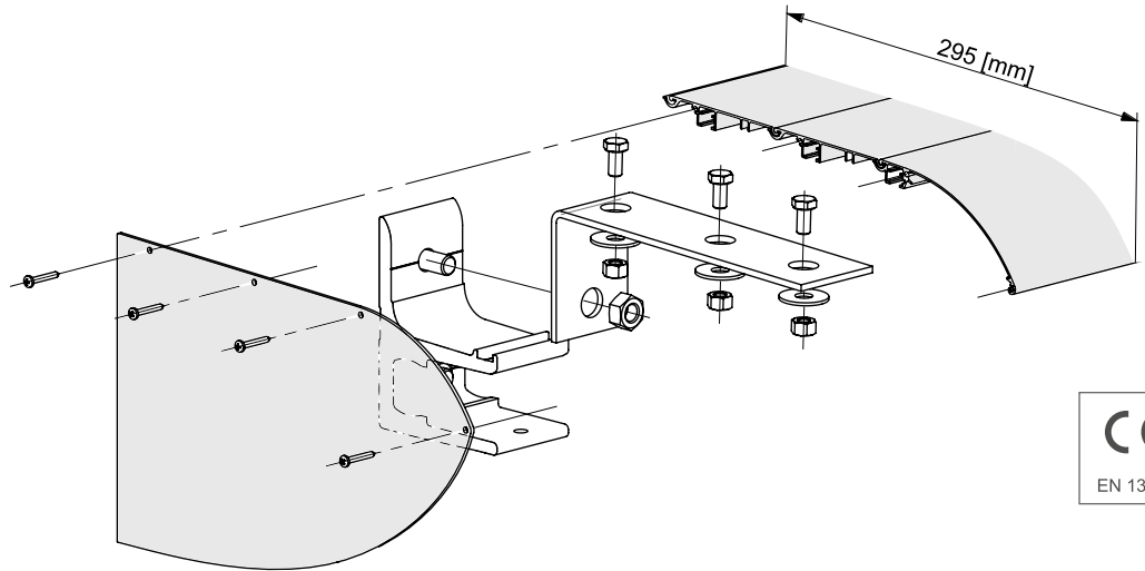
Hood before assembling
