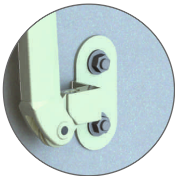
Side bracket (inside the recess)
